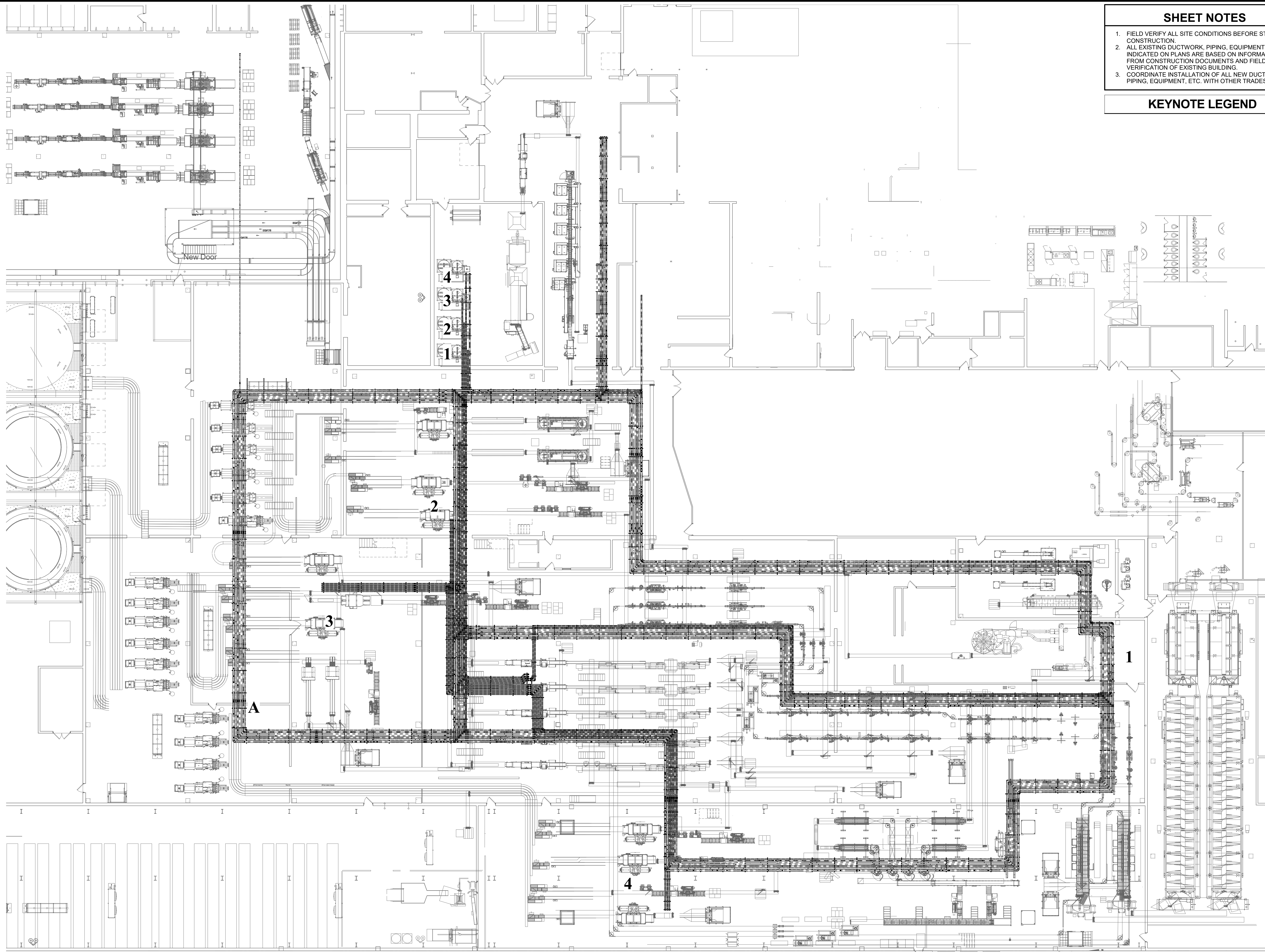
1 OVERALL PROCESS PIPING PLAN 1/16" = 1'-0"
